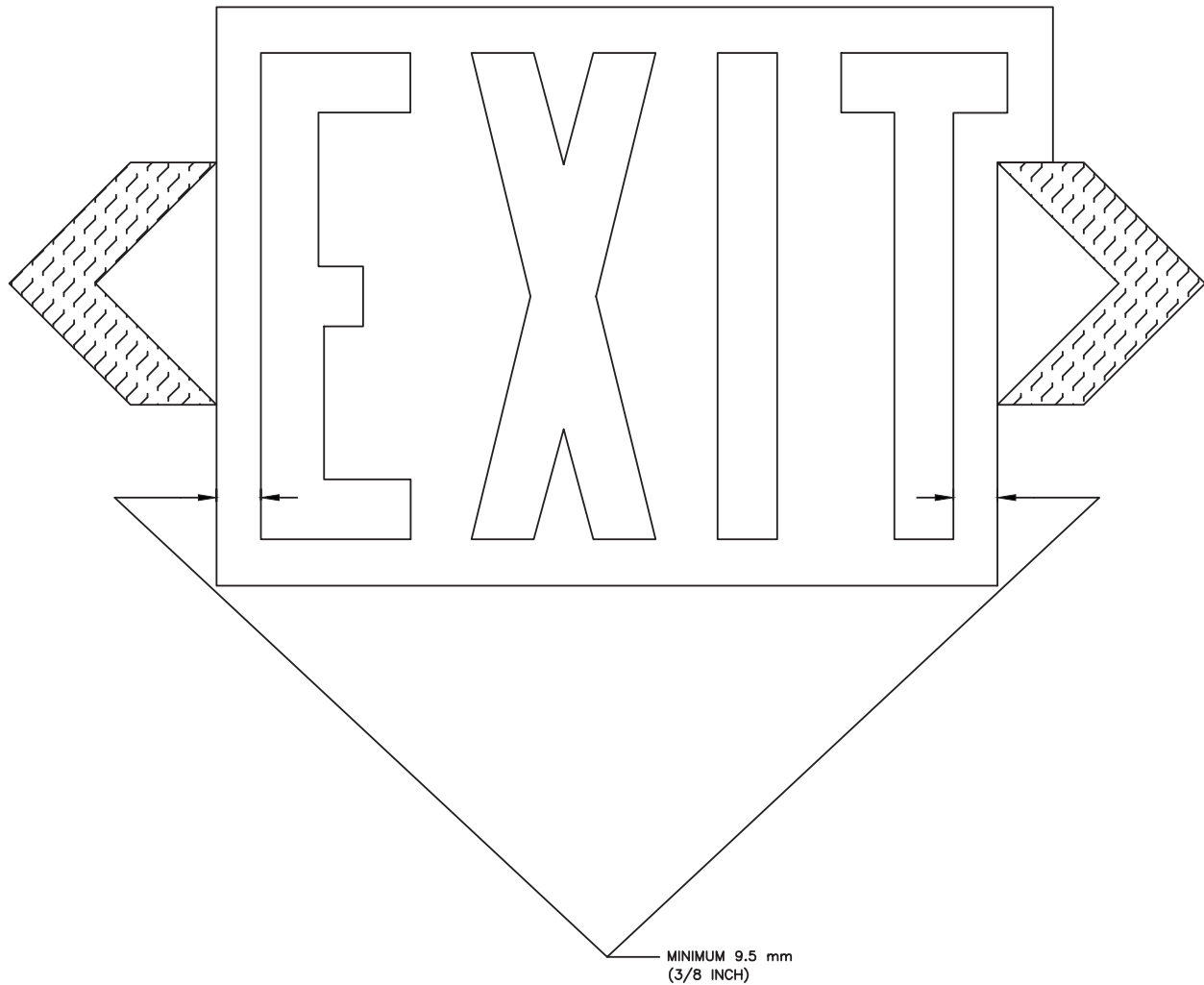
FIGURE 2 — MINIMUM DISTANCE BETWEEN DIRECTIONAL INDICATOR AND LEGEND
